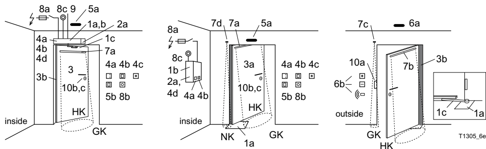
iMotion 1301, 1301.S
